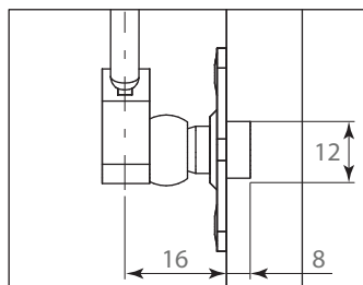
Enganche lateral
