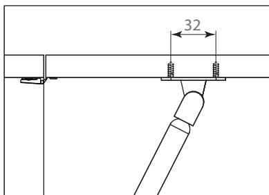
Enganche frontal
